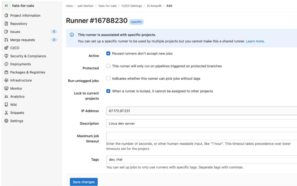
Figure 5.7 – Runner settings in the GitLab UI
