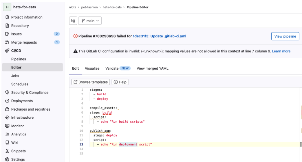
Figure 12.3 – Pipeline Editor showing an invalid CI/CD configuration
